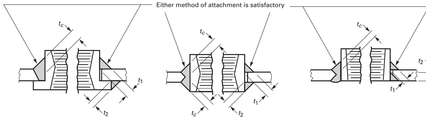
Figure UW-16.1 Some Acceptable Types of Welded Nozzles and Other Connections to Shells, Heads, etc. (Cont'd)
