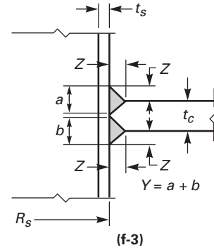
Figure 9-5 Some Acceptable Types of Jacket Closures (Cont'd)
