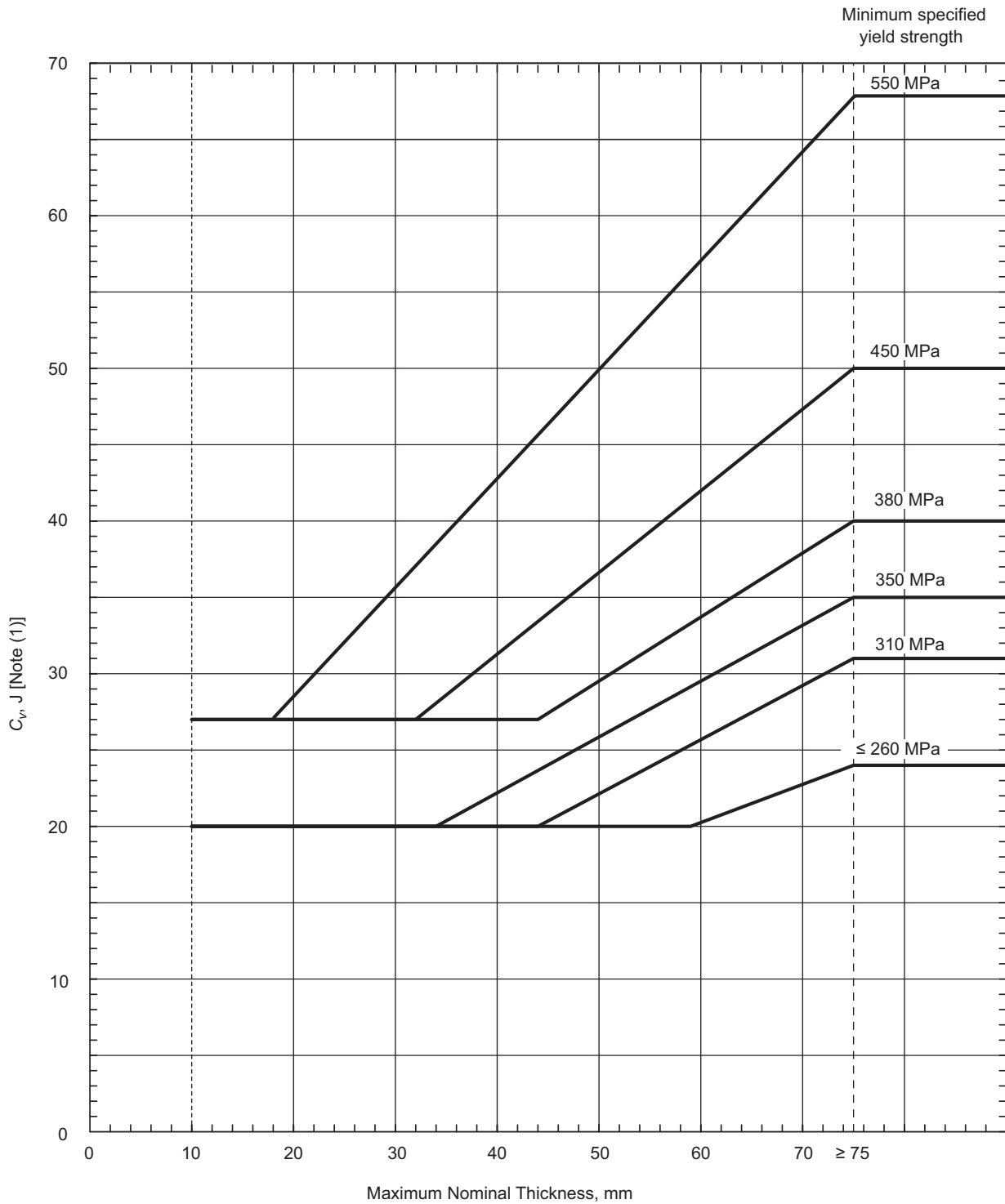
Figure UG-84.1M Charpy V-Notch Impact Test Requirements for Full-Size Specimens for Carbon and Low Alloy Steels, Having a Specified Minimum Tensile Strength of Less Than 655 MPa, Listed in Table UCS-23
