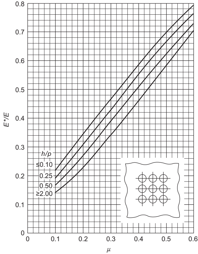
(a) E^*/E (Square Pattern)
