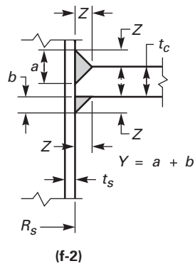
Figure 9-5 Some Acceptable Types of Jacket Closures (Cont'd)
