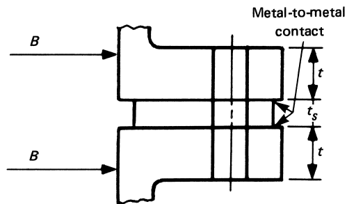
(b) Integral With Spacer [See Note (1)]
