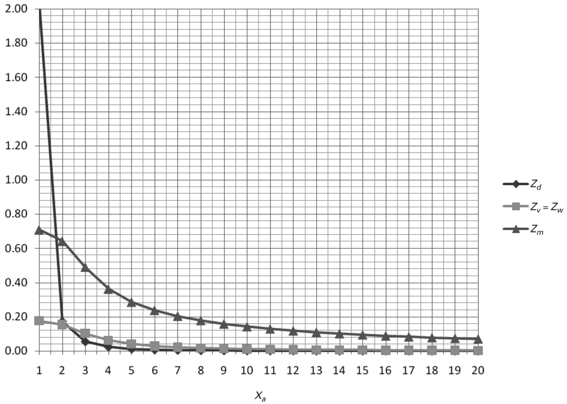
Figure LL-1-1 Z_v, Z_d, Z_w, and Z_m Versus X_a
