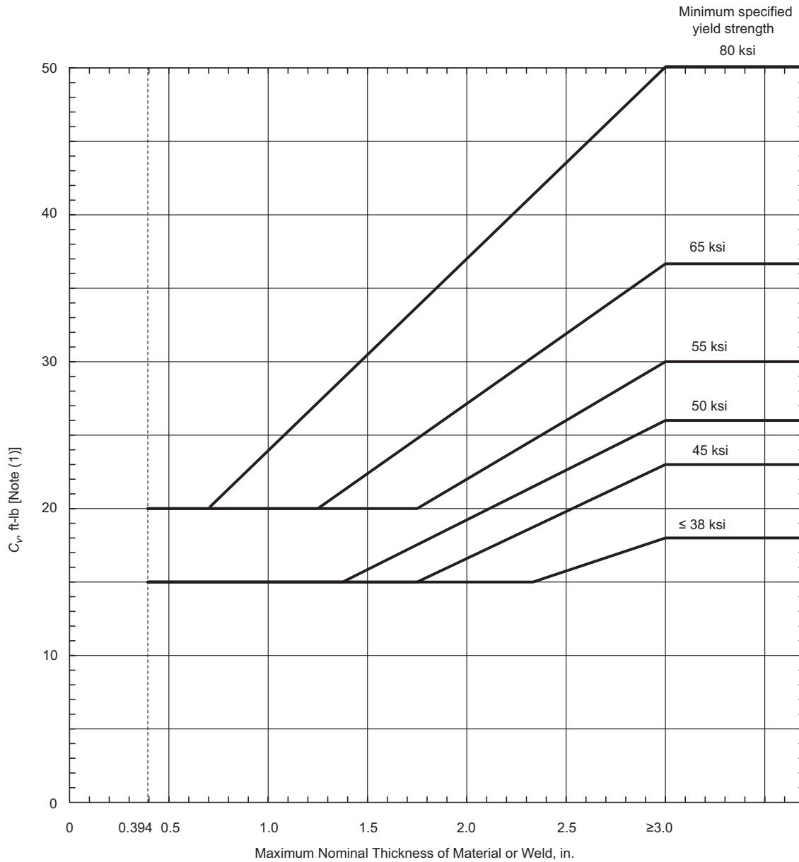
Figure UG-84.1 Charpy V-Notch Impact Test Requirements for Full-Size Specimens for Carbon and Low Alloy Steels, Having a Specified Minimum Tensile Strength of Less Than 95 ksi, Listed in Table UCS-23
