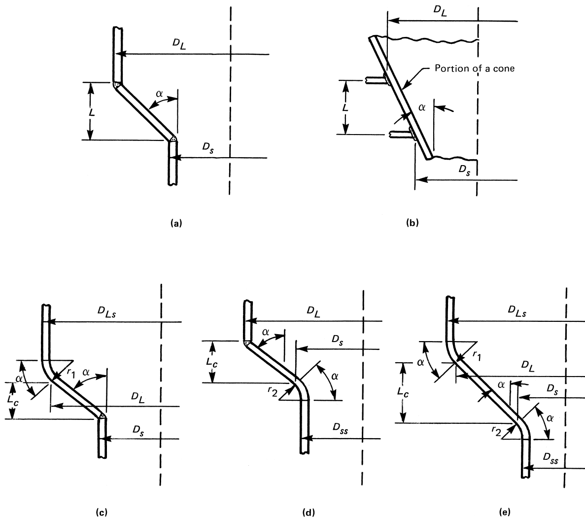
Figure UG-33.1 Length L_c of Some Typical Conical Sections for External Pressure
