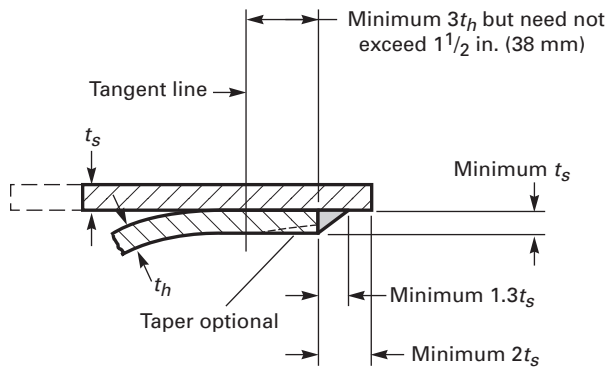
Figure UW-13.1 Heads Attached to Shells (Cont'd)
