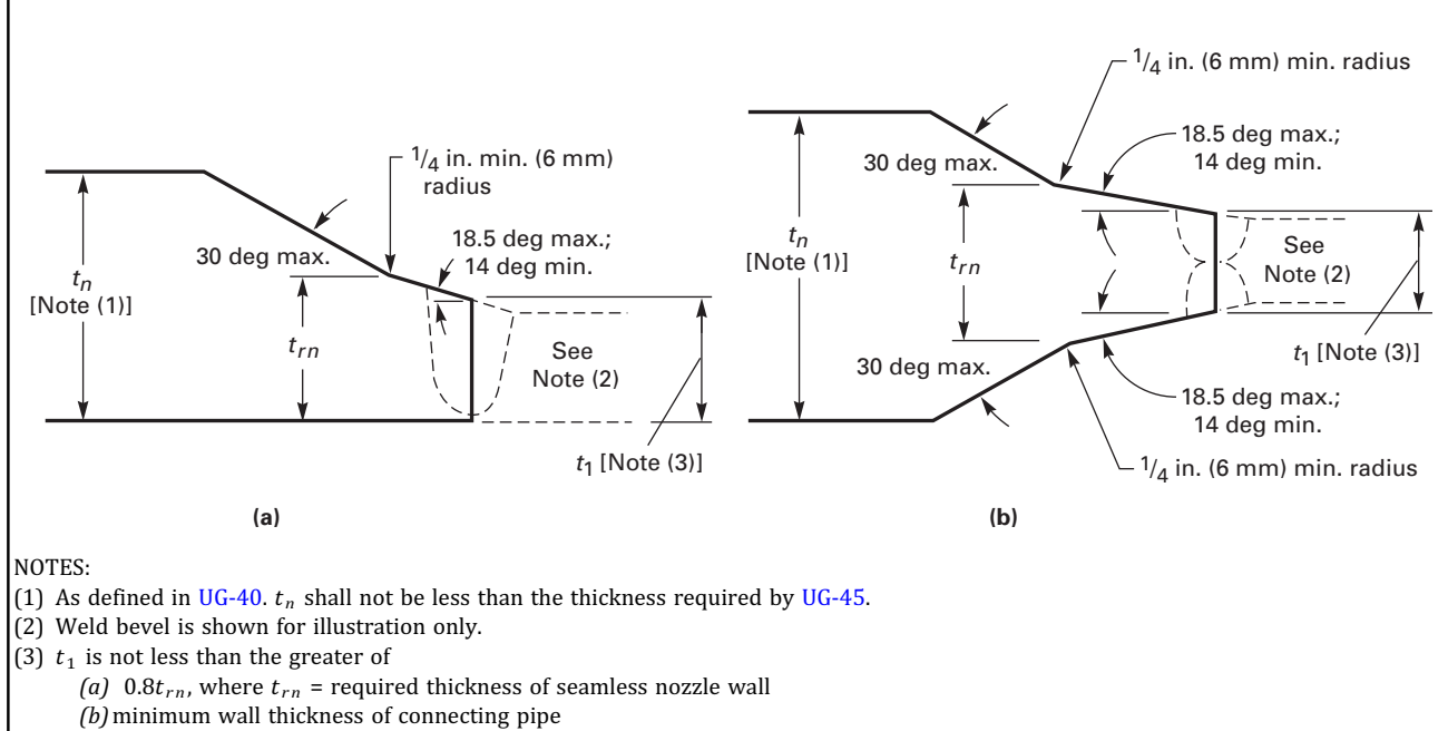
Figure UW-13.4 Nozzle Necks Attached to Piping of Lesser Wall Thickness
