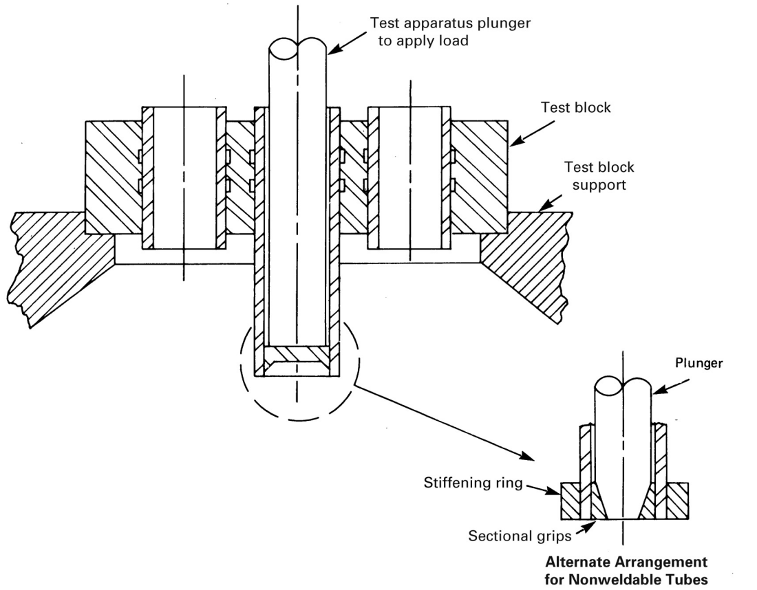
Figure UW-20.3 Typical Test Fixtures for Expanded or Welded Tube-to-Tubesheet Joints
