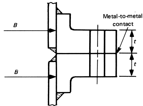
(c) Loose-Type With Hub [See Note (2)]
