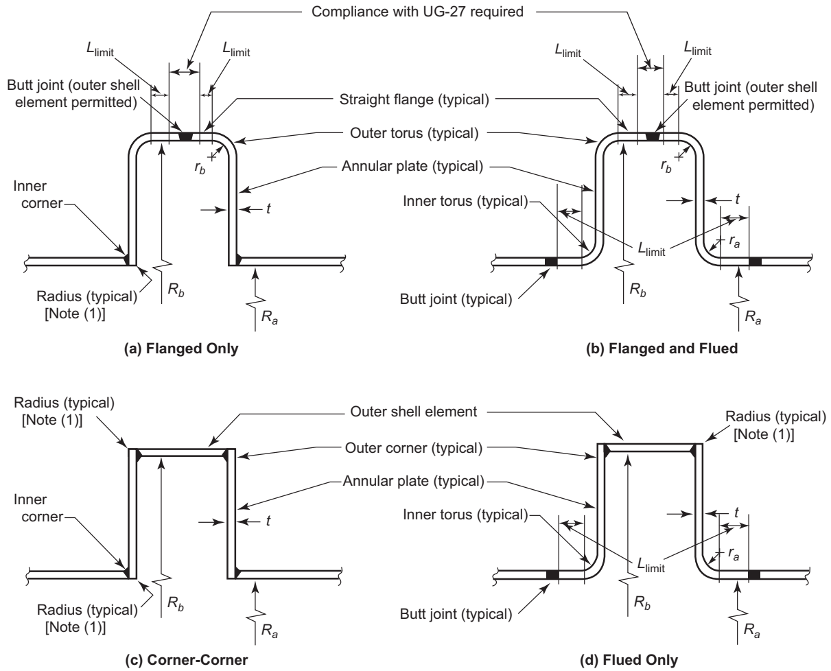
Figure 5-1 Typical Flexible Shell Element Expansion Joints
