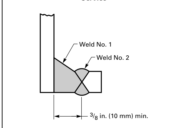
Figure UW-13.5 Fabricated Lap Joint Stub Ends for Lethal Service
